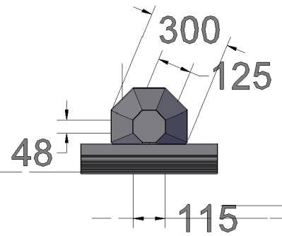
LIGHT POST top view
