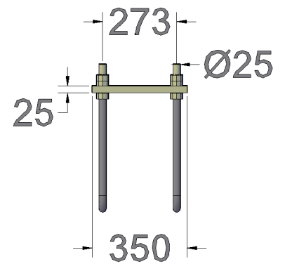
MAST FLANG front view
