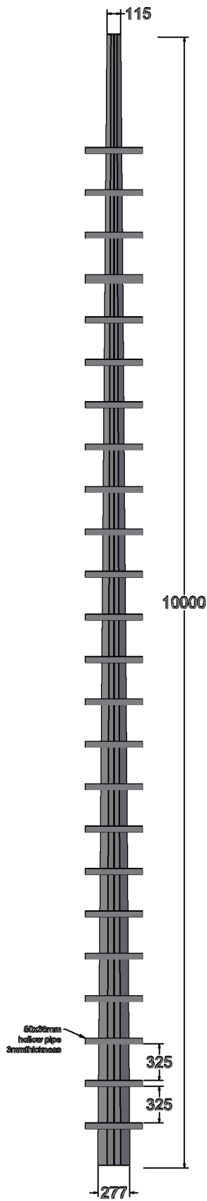
LIGHT POST front view
