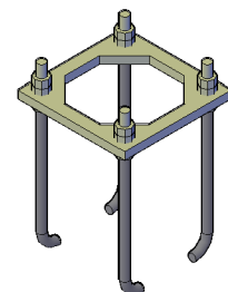
MAST FLANG isometric view
