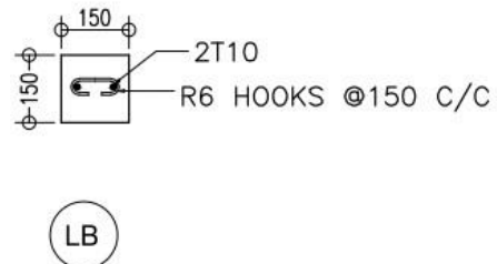
LINTEL /SILL BEAMS
