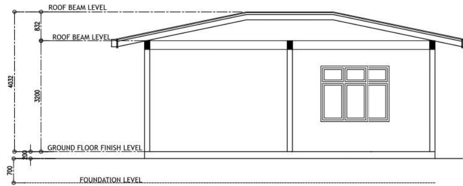
SECTION X-X SCALE - 1:100
