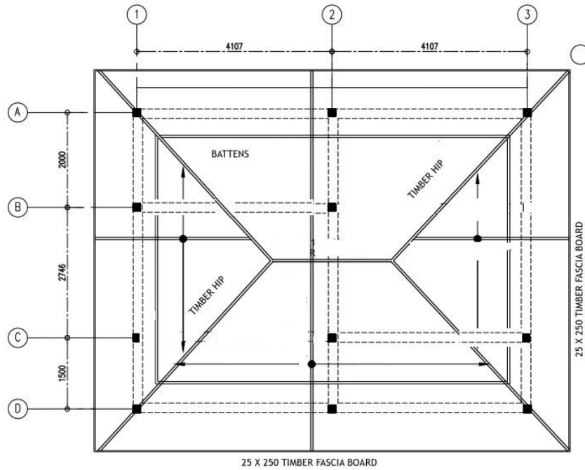
ROOF FRAMING PLAN SCALE - 1:100
