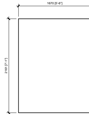
Ramp Details
