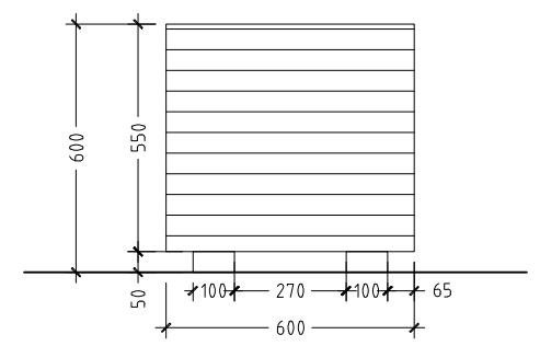
PB2 ELEVATION - A SCALE 1:20
