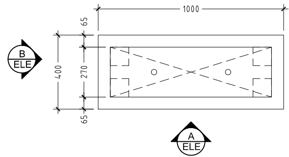
PLANTER BOX 3 - PLAN PB3 SCALE 1:20
