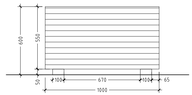
PB1 ELEVATION - A SCALE 1:20
