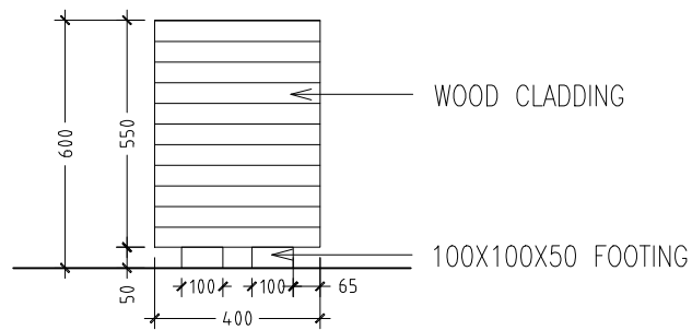
ELEVATION - B PB3 SCALE 1:20
