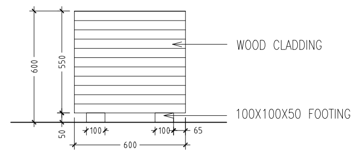
PB2 ELEVATION - B SCALE 1:20
