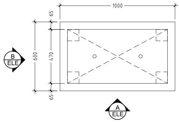
PB1 PLANTER BOX 1 - PLAN SCALE 1:20
