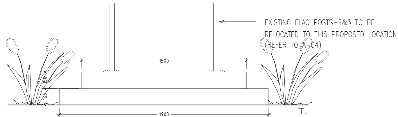
FLAG POST - ELEVATION A SCALE 1:20
