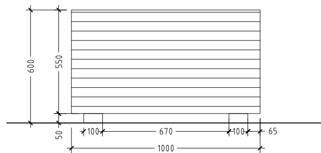
ELEVATION - A PB3 SCALE 1:20
