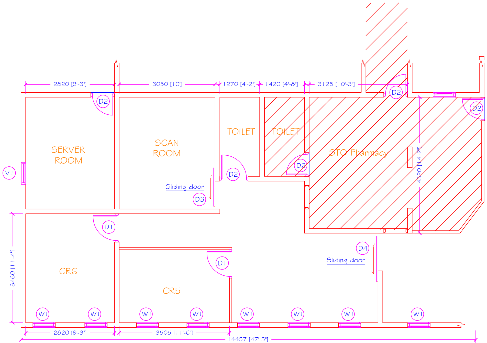
OPD EXTENSION FLOOR PLAN
