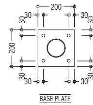
BASE PLATE
