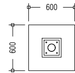
FOOTING DETAILS 1:50
