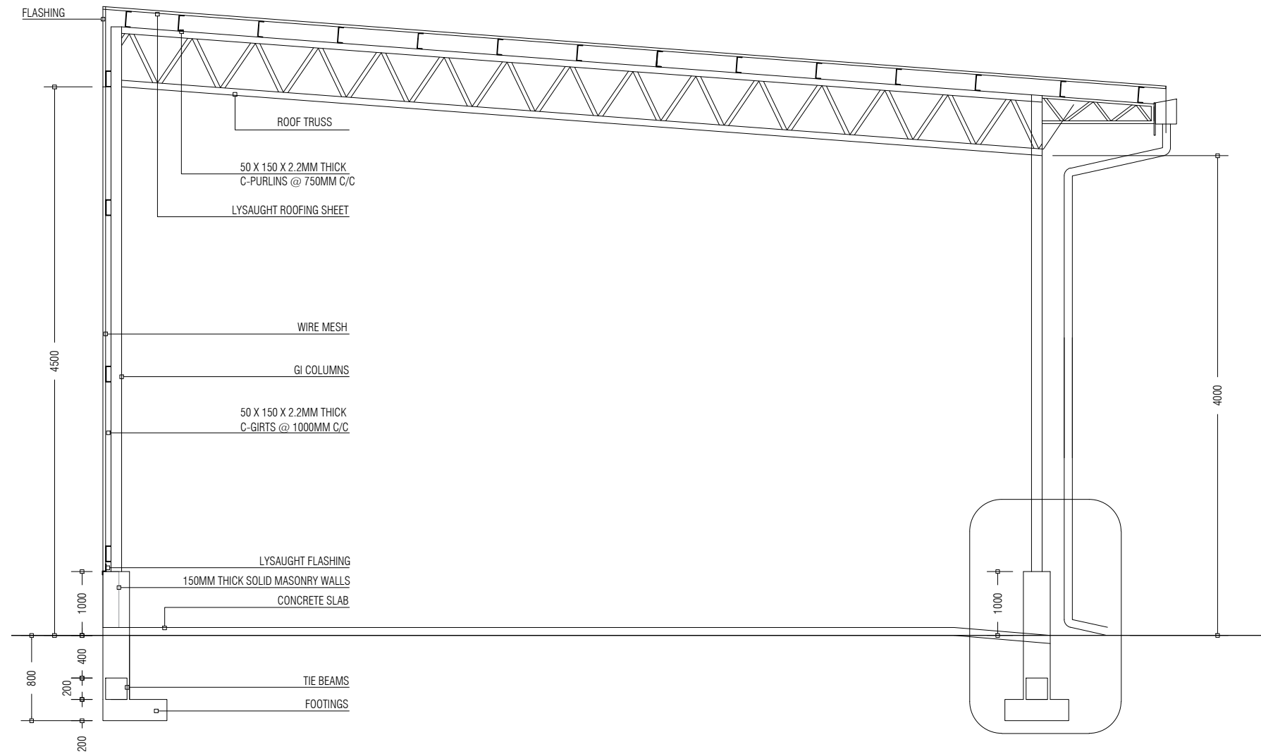
WASTE MANAGEMENT BAY SECTION
