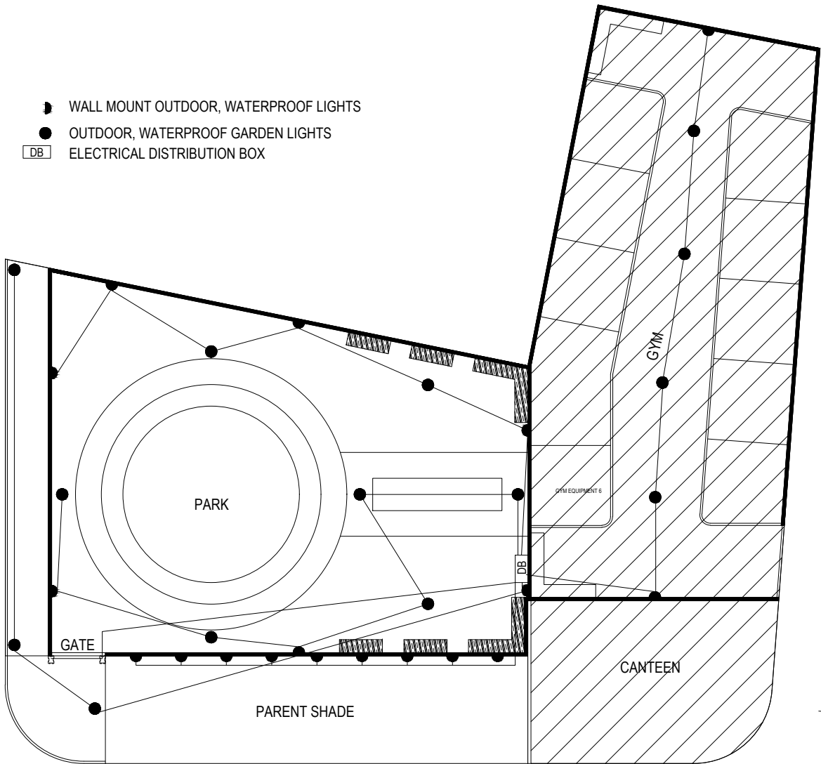
ELECTRC LAYOUT
