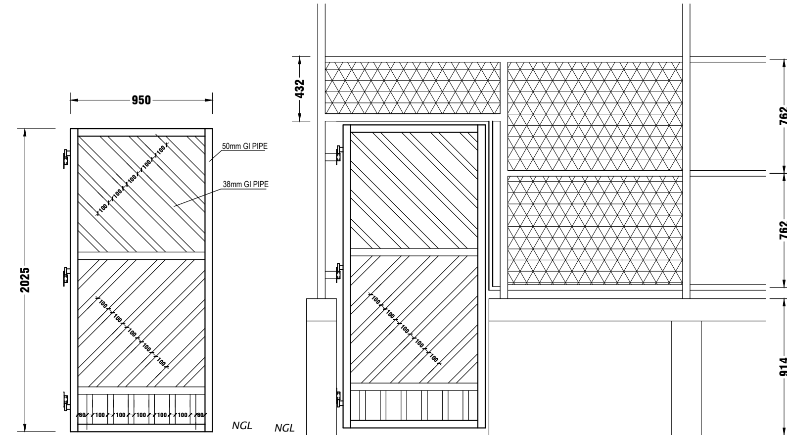
GATE -B DETAIL
