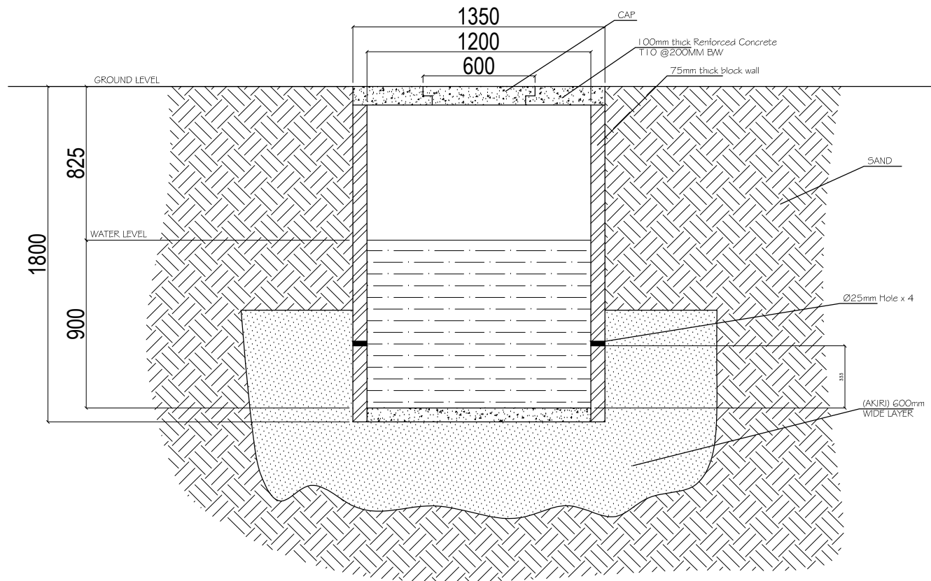
WELL DETAIL
