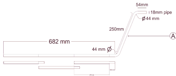
BACK LEG 3 Extending poles
