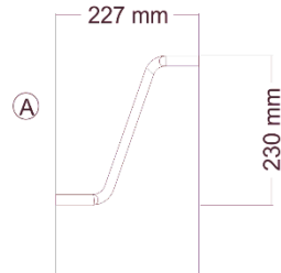
DETAIL VIEW OF BEND PIECE OF REAR LEG
