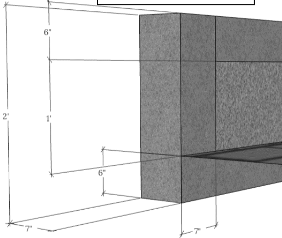
Boundary Wall Details
