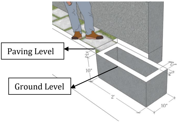
Junction box measurement
