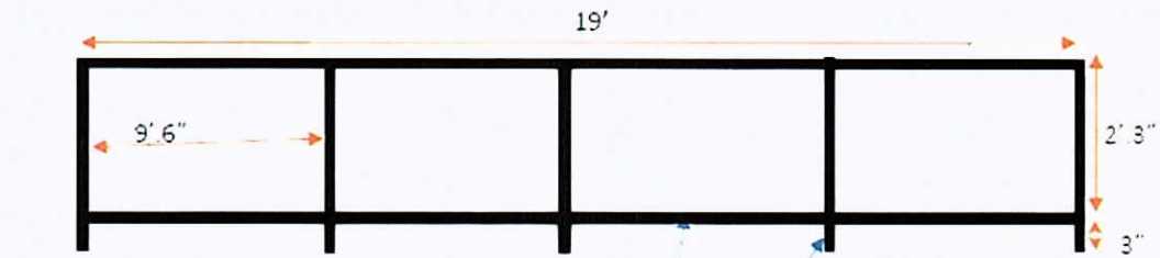
FRONT/BACK VIEW (without two side top fence)
