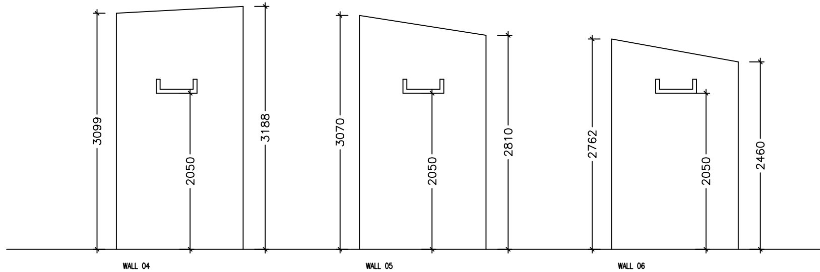
DETAIL 01 - ELEVATION 1:50
