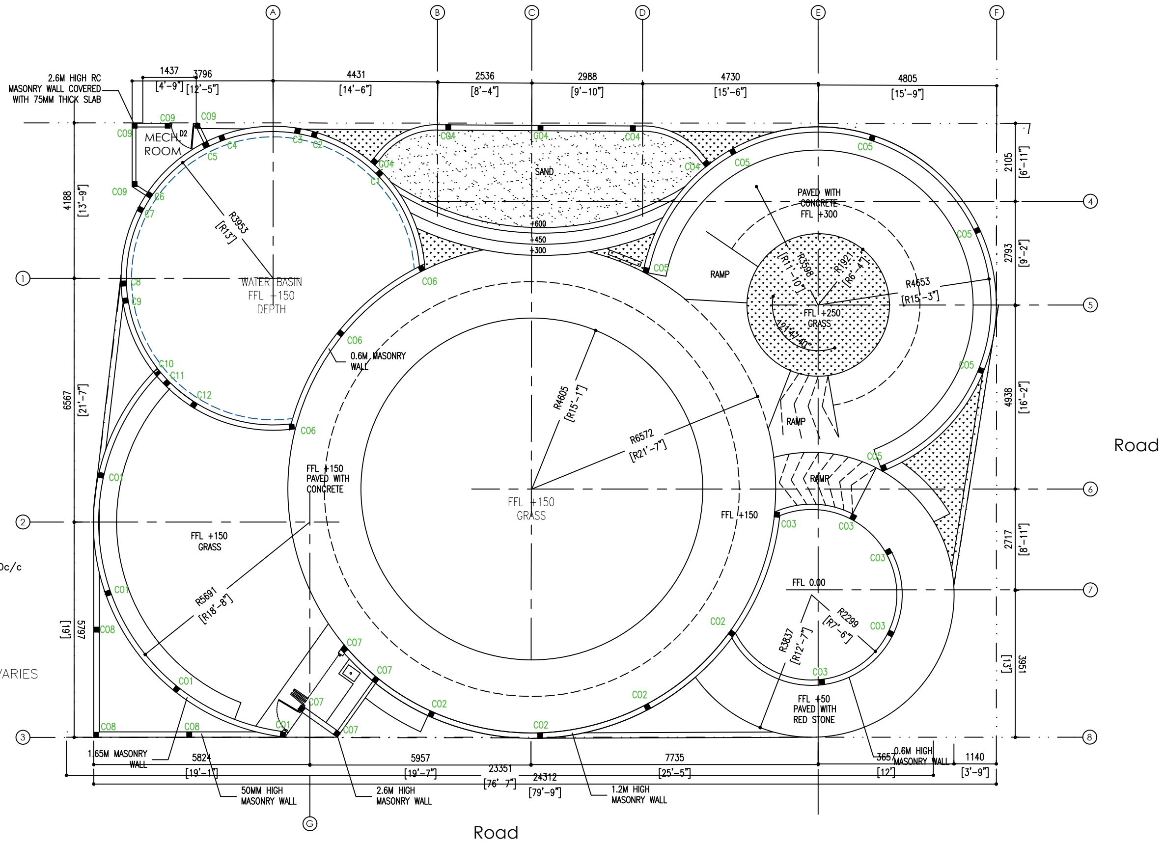
COLUMN PLAN 1:100
