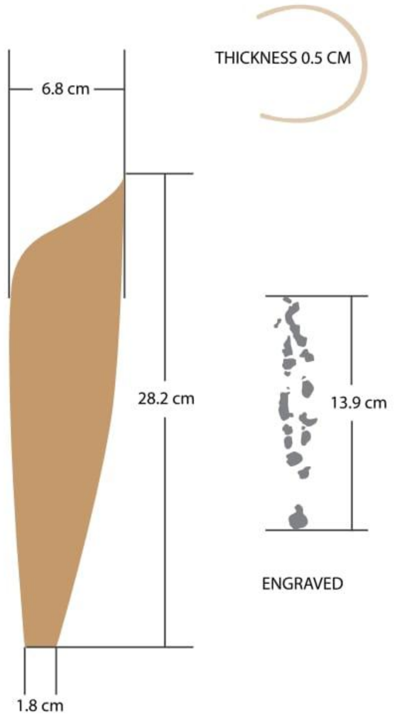
TOP VIEW OF GOLD SECTION
