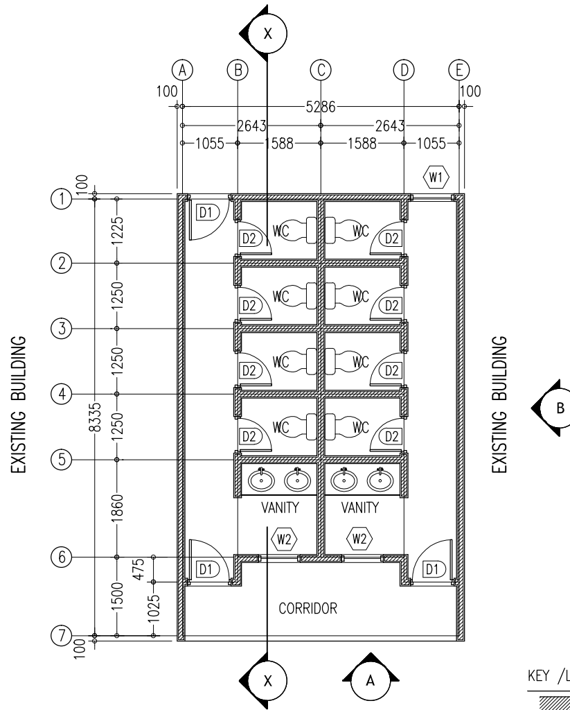
FLOOR LAYOUT PLAN SCALE 1:100
