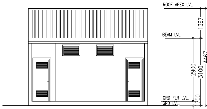
ELEVATION-A SCALE 1:100
