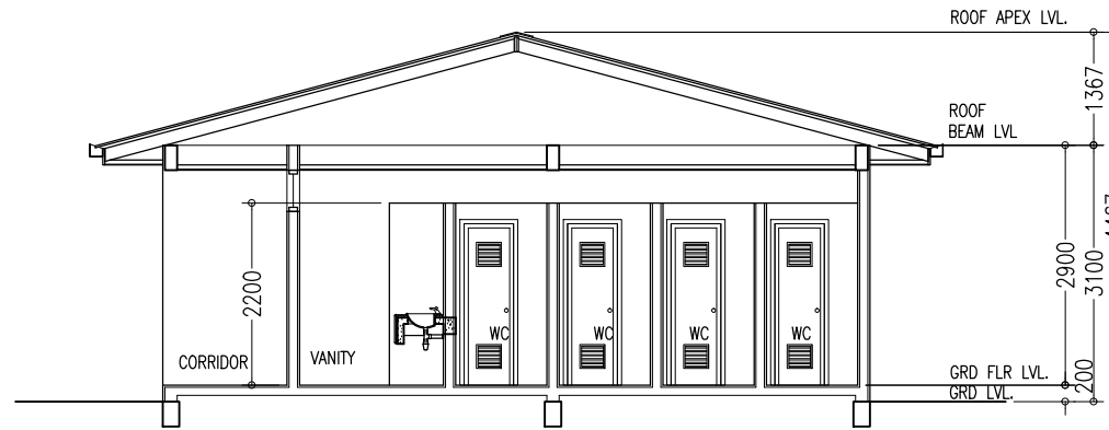
SECTION X-X SCALE 1:100
