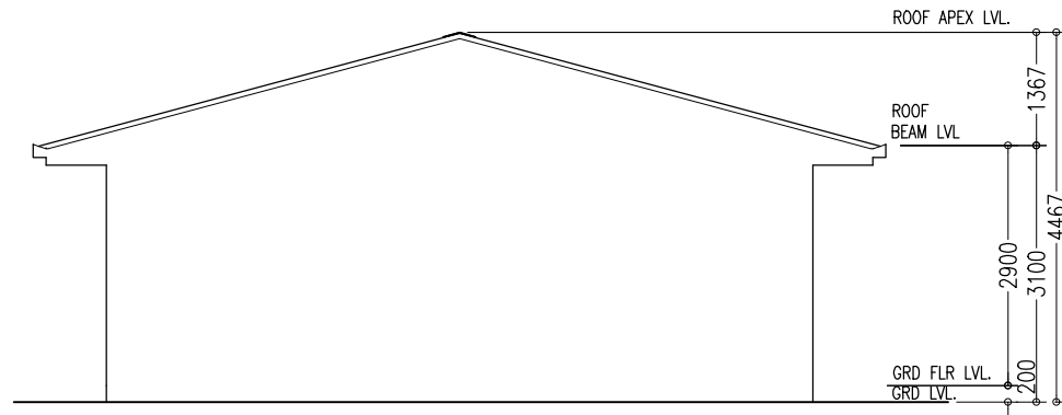
ELEVATION-B SCALE 1:100
