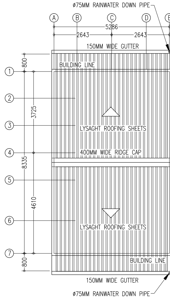
ROOF STRUCTURE PLAN SCALE 1:100
