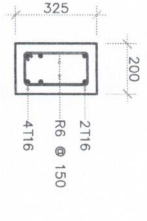
MIDSPAN 1:20
