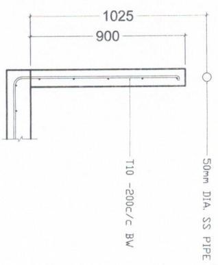
TYPICAL BALCONY DETAILS SCALE: 1:20
