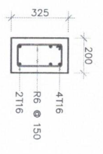
SUPPORT 1:20
