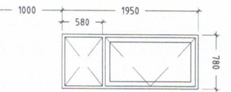
WINDOW W2 1:50
