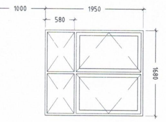
WINDOW W1 1:50
