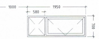
WINDOW W5 1:50
