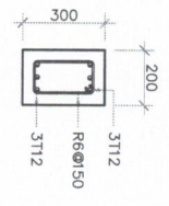
TIE BEAM TB 1:20
