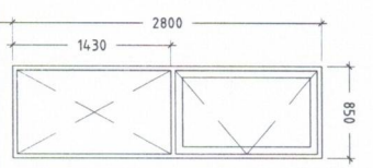
WINDOW W3 1:50
