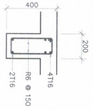
FLOOR BEAM B2 1:20
