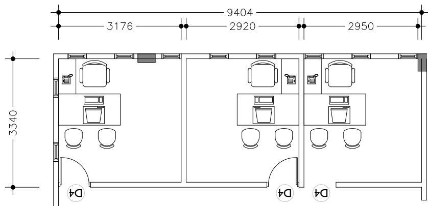
STATE MINISTER ROOM SCALE 1:100
