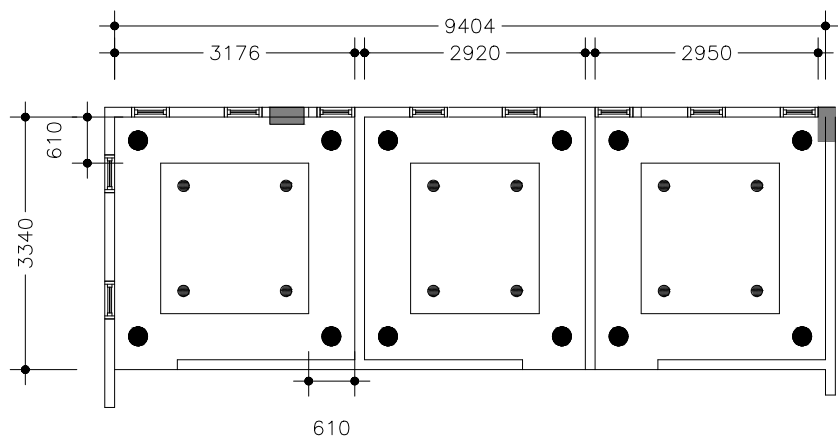
STATE MINISTER ROOM CEILING PLAN SCALE 1:100
