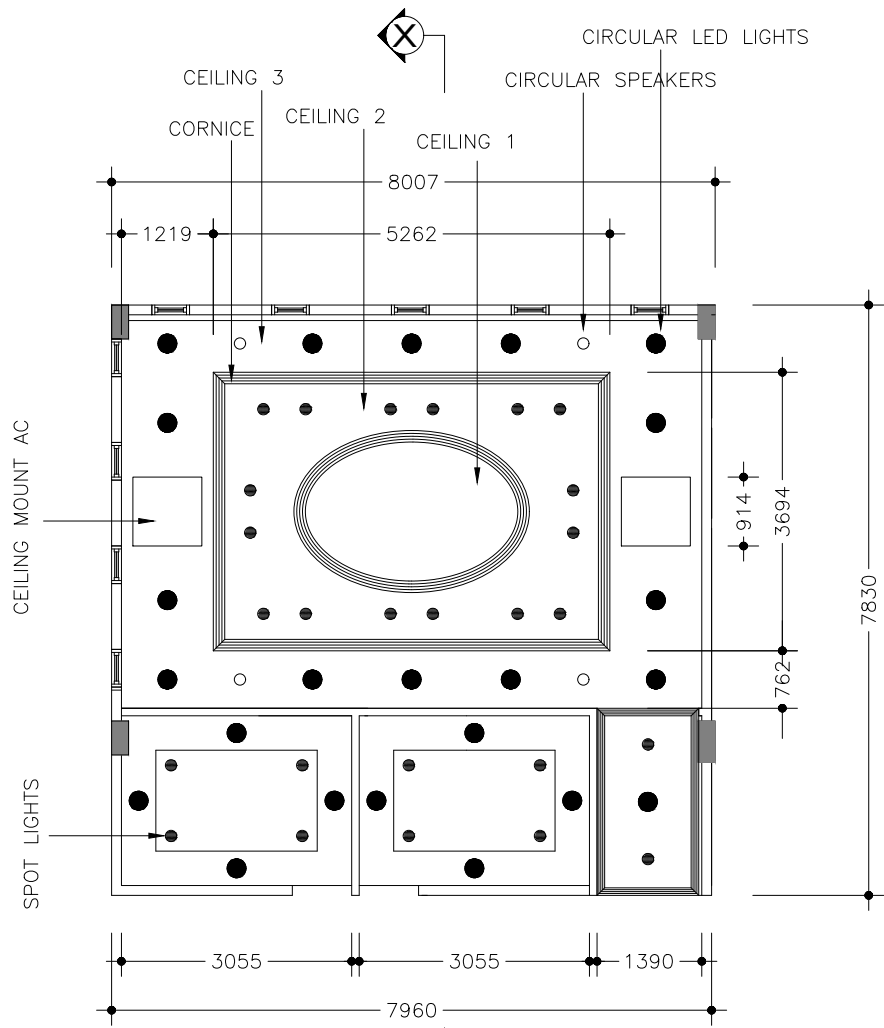
MEETING ROOM CIELING PLAN SCALE 1:100
