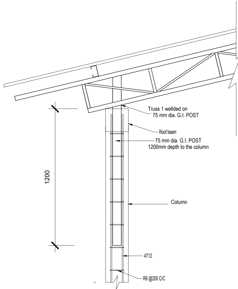
Cloumn Post and truss Fixing Detal
