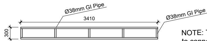
TRUSS 2 DETAIL
