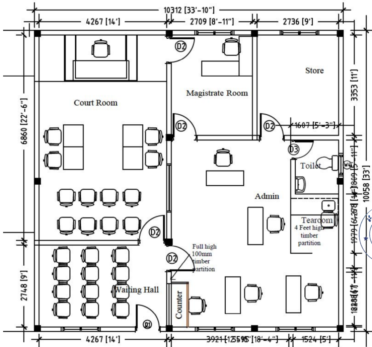
FLOOR PLAN SCALE 1:75
