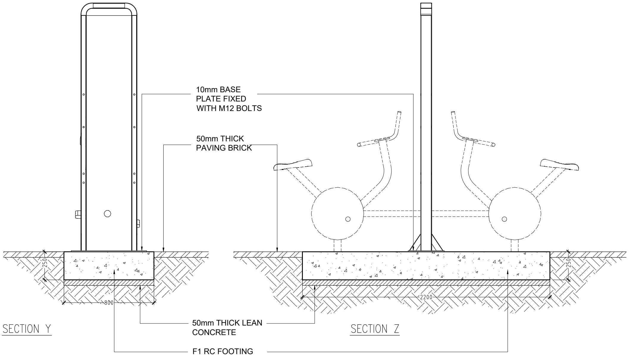
EQUIPMENT FIXING DETAIL [D2]
