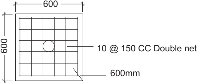
FOOTING
