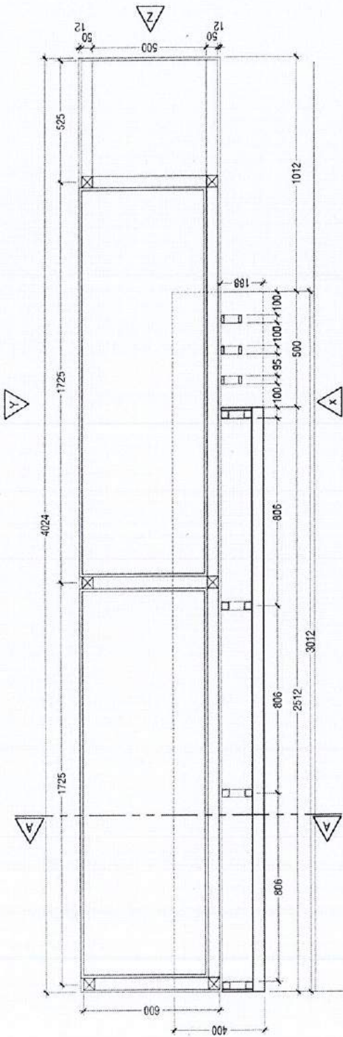
RECEPTION DESK PLAN
