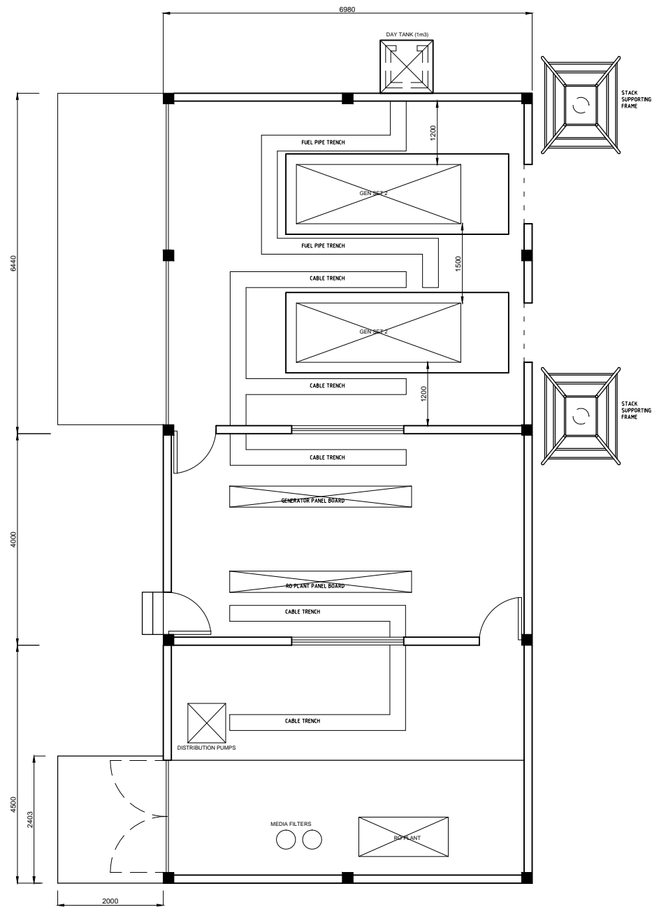
FLOOR PLAN
