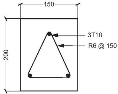
FOUNDATION BEAM
