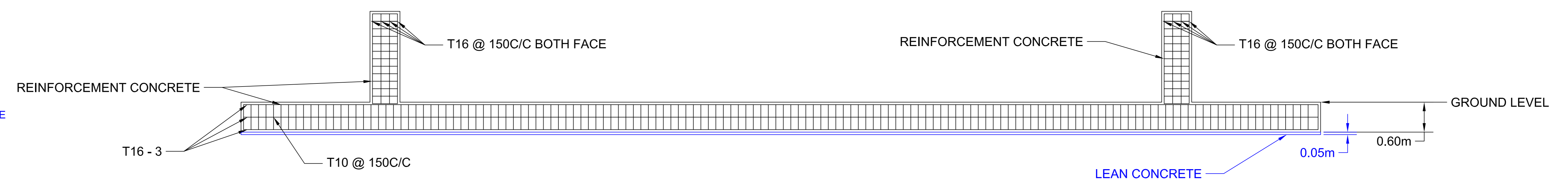
FRONT VIEW
