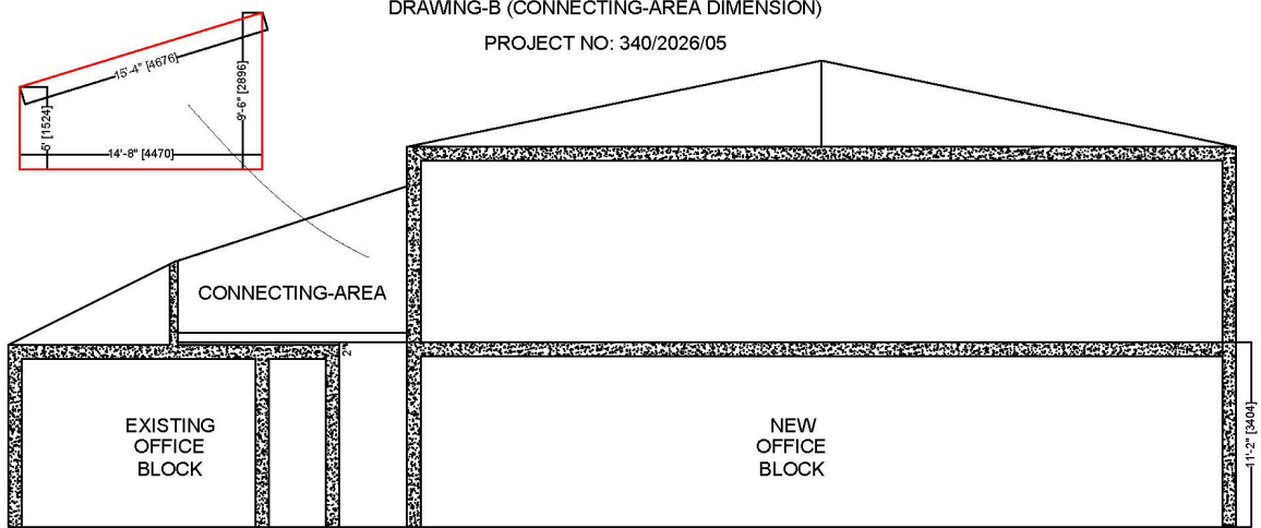
DRAWING-B (CONNECTING-AREA DIMENSION)
