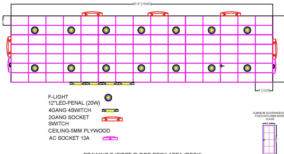
DRAWING-F (FIRST-FLOOR-DECK-AREA (DECK))
