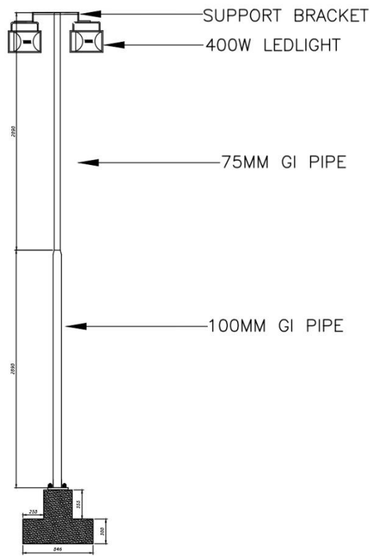
DETAIL LIGHT POST Scale - 1:30
