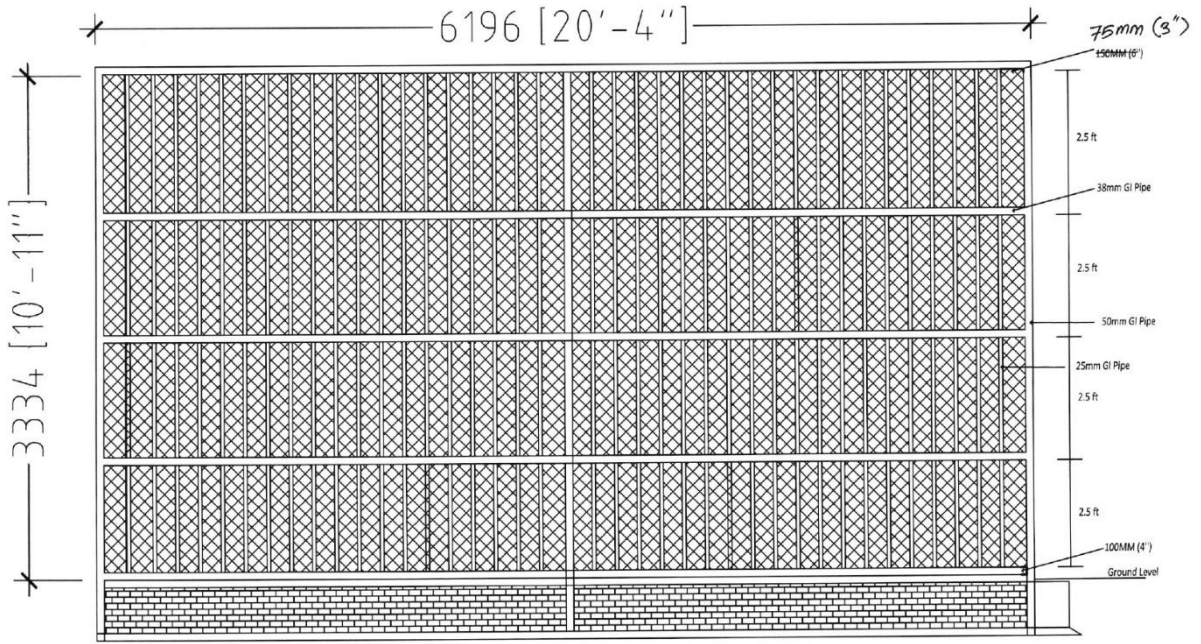
FUTSAL GROUND GOAL FENCING DETAIL SCALE 1:25
