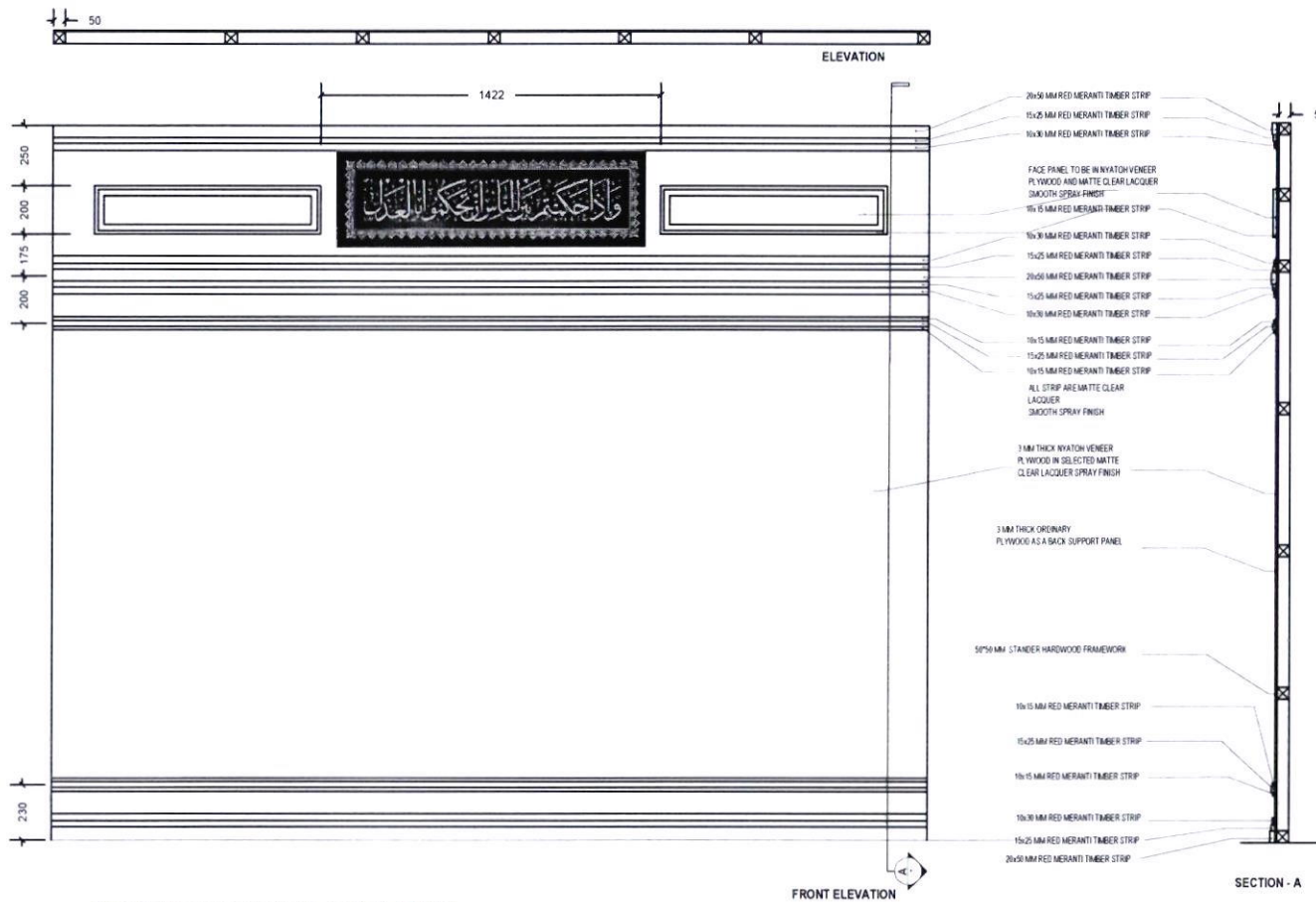
COURT ROOM BACK PANEL SCALE 1:30
