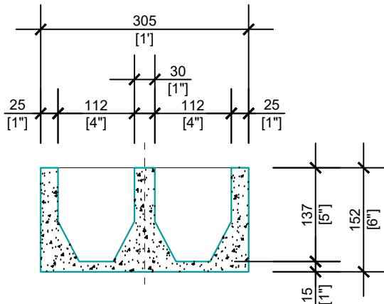
SECTION DETAILS
