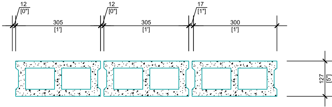
WALL PLAN
