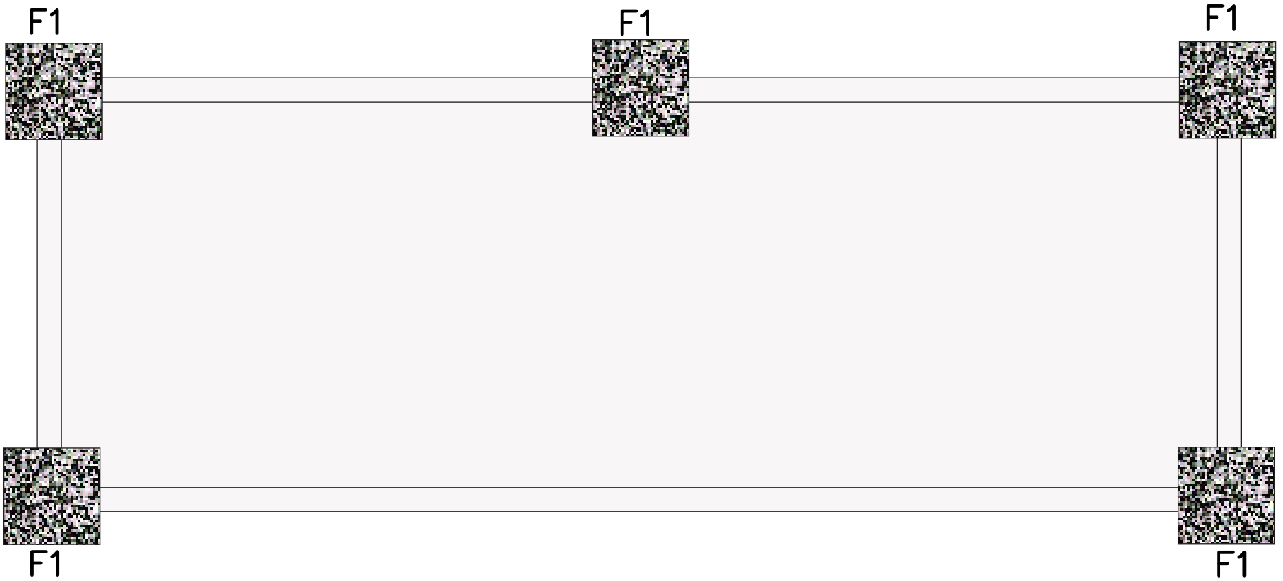
FOUNDATION PLAN
