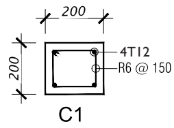
COLUMN DETAILS
