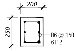
FOUNDATION DETAILS
