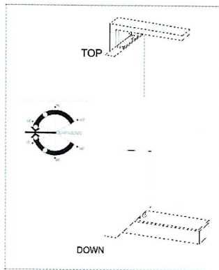
Double Action Floor Spring Hinge
