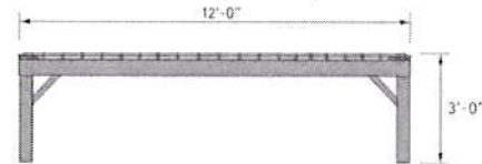
FRONT VIEW (ELEVATION)
