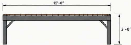
FRONT VIEW (ELEVATION)
