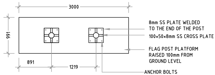
FLAG POST DETAIL (PLAN) SCALE 1:50
