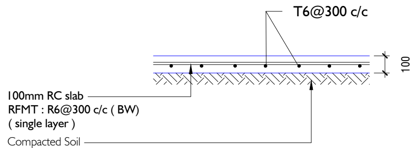
TYPICAL GROUND SLAB DETAIL SCALE 1:20
