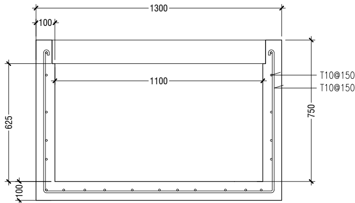
PUMP BOX UNDERGRAD
