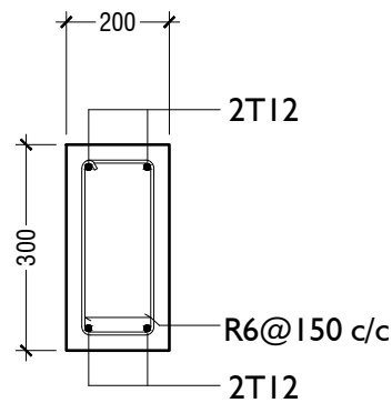
BEAM 'TB' SCALE 1:20
