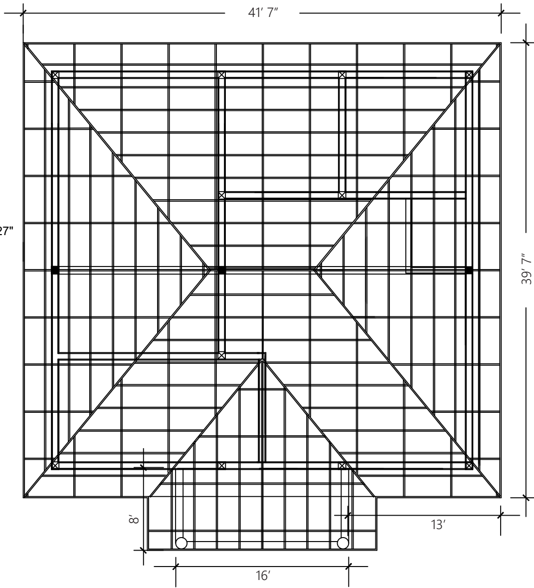
ROOF STRUCTURE LAYOUT
