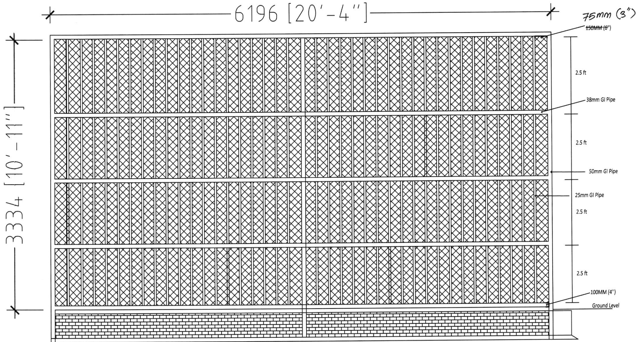
FUTSAL GROUND GOAL FENCING DETAIL
