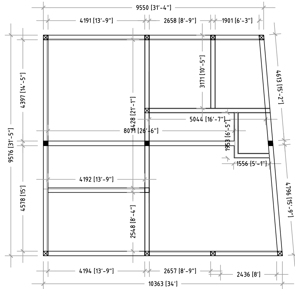
ROOFBEAM LAYOUT SCALE 1:100
