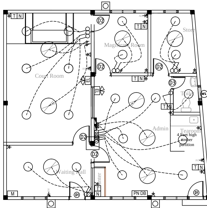
ELECTRICAL LAYOUT SCALE 1:100
