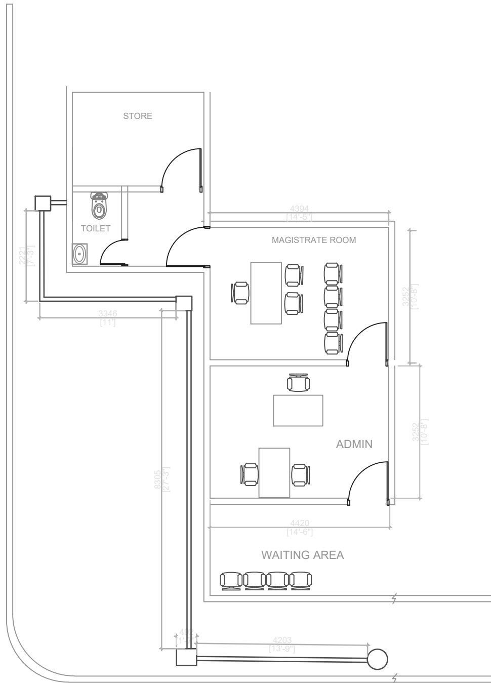
THINADHOO COURT FLOOR PLAN SCALE 1:200
