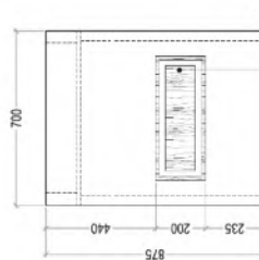
FRONT ELEVATION
