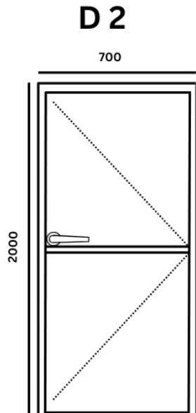
SWING DOOR FRAME = A + PANEL = A.C IRONMONGERY = S.S
