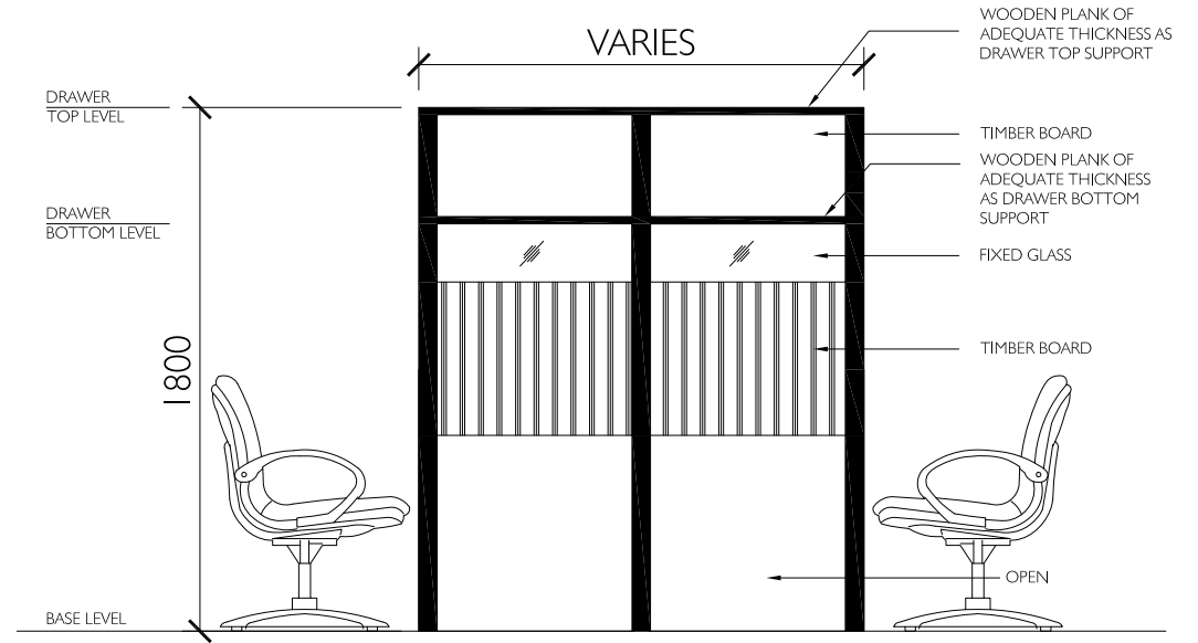
TYPICAL WORKSTATION SIDE ELEVATION NOT TO SCALE
