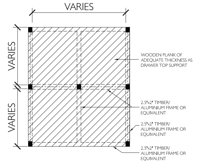
TYPICAL DRAWER TOP PLAN NOT TO SCALE
