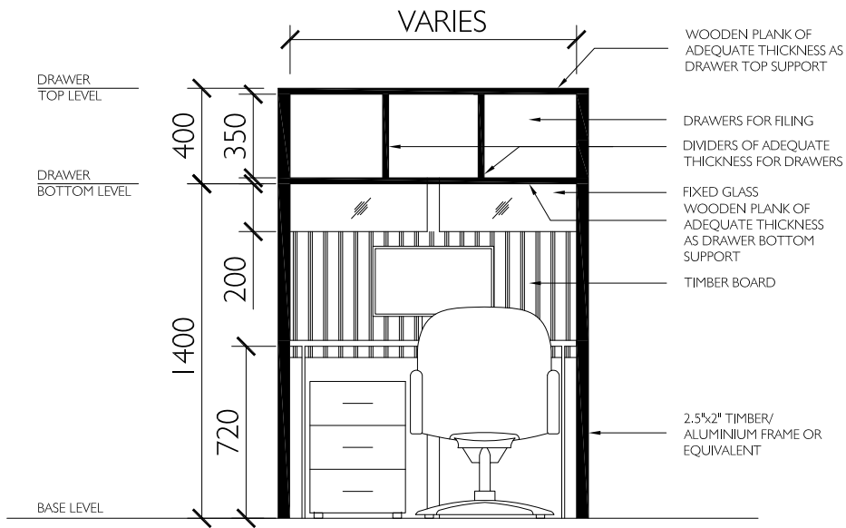
TYPICAL WORKSTATION FRONT ELEVATION NOT TO SCALE
