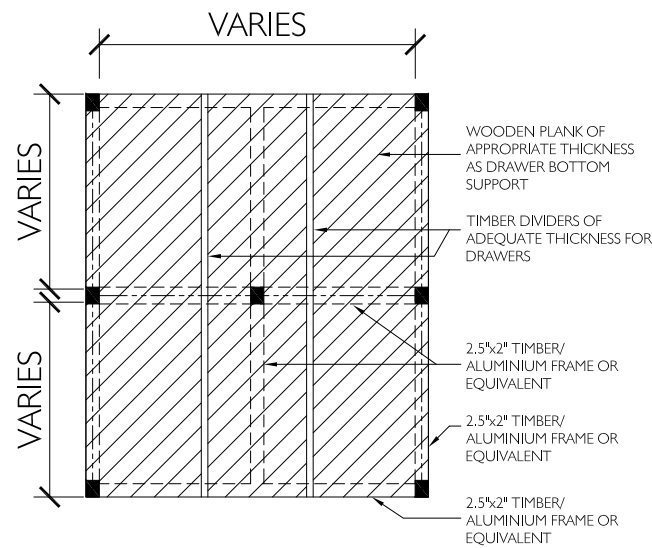
TYPICAL DRAWER BOTTOM PLAN NOT TO SCALE
