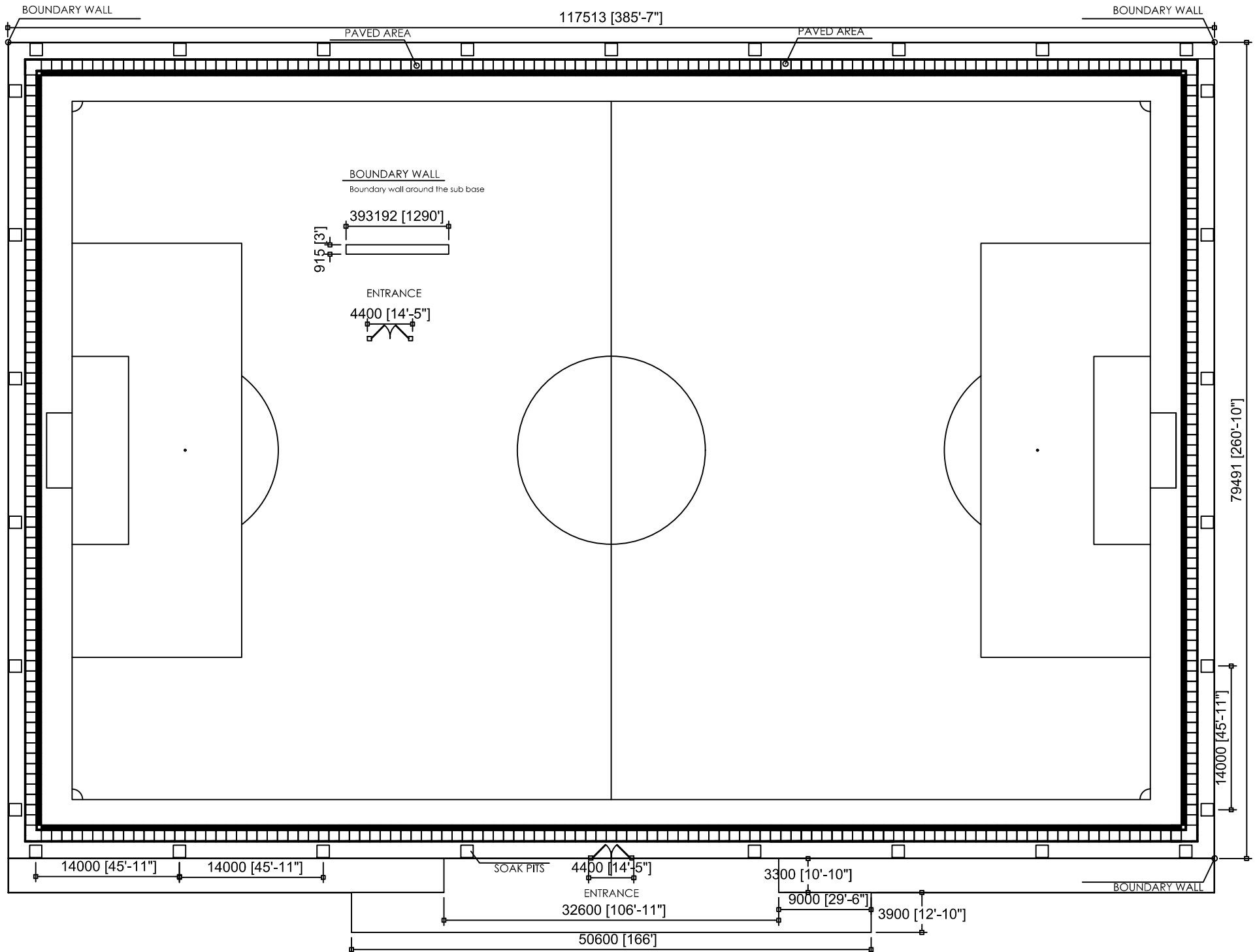
○ STANDARD ARTIFICIAL TURF FULL PITCH PLAN
