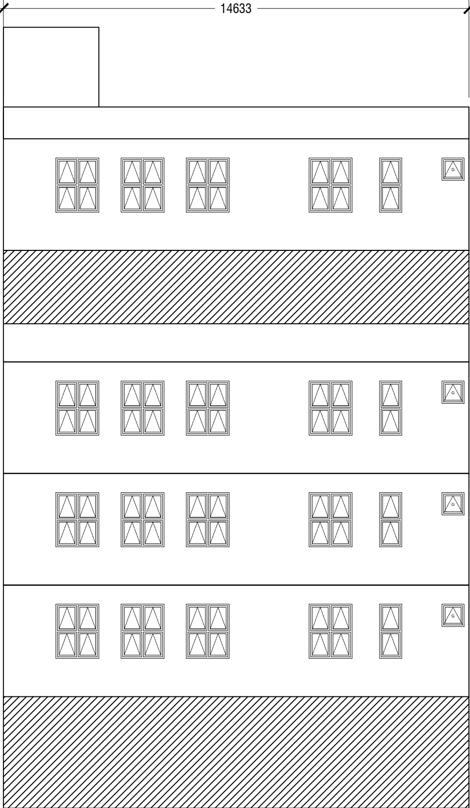
ELEVATION E2 HATCHED AREA SEALER NOT REQUIRED
