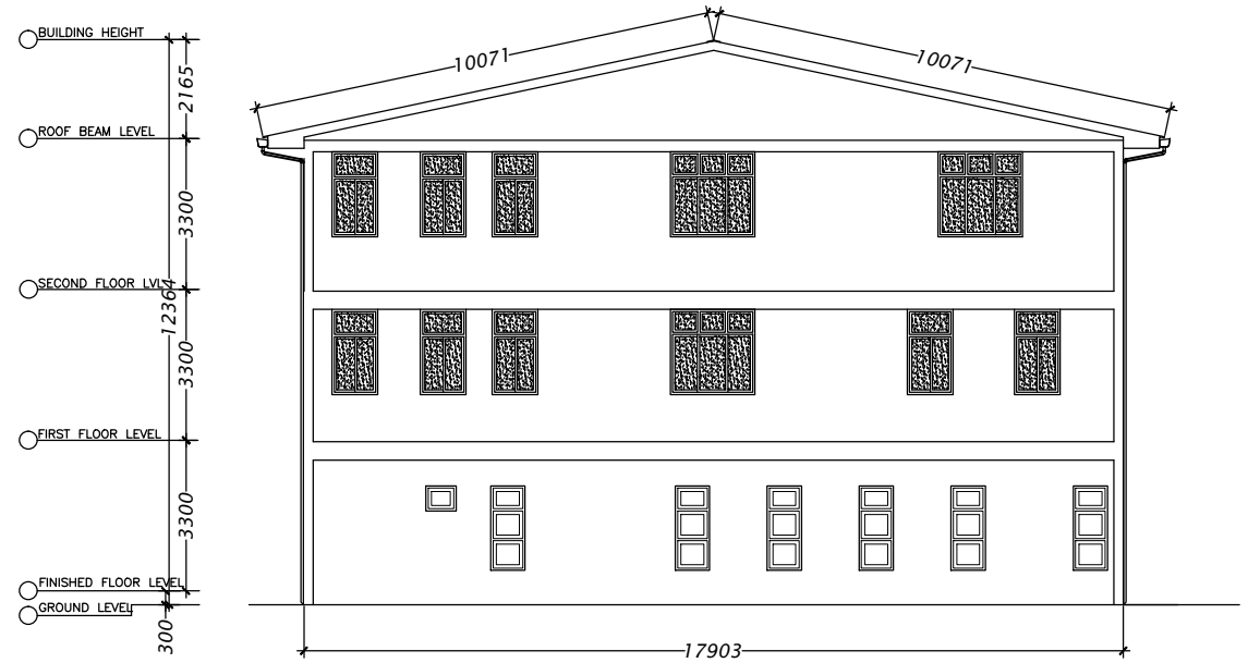
OFFICE BUILDING
