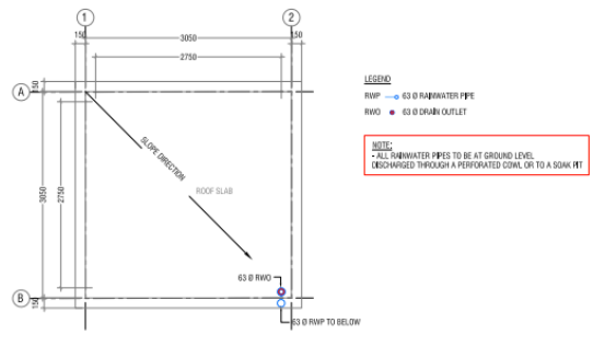
SECURE ROOM - DRAINAGE LAYOUT SCALE 1:50
