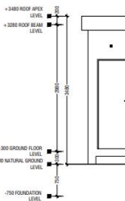
ELEVATION A-A SCALE 1:50
