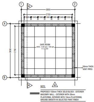
VENT PIPE - PLAN (+2800) SCALE 1:50
