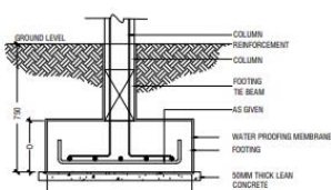
SECTION FOOTING DETAILS SCALE 1:20
