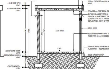
SECTION A-A SCALE 1:50
