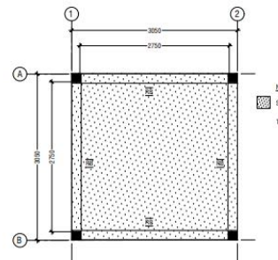
ROOF BEAM & SLAB PLAN SCALE 1:50
