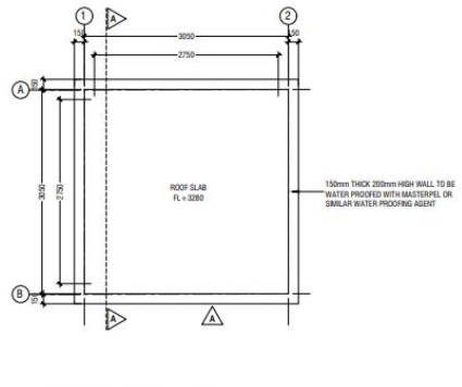
SECURE ROOM - PLAN SCALE 1:50
