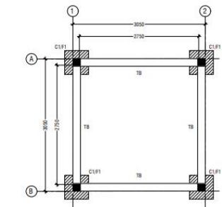
FOUNDATION - PLAN SCALE 1:50
