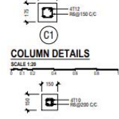
COLUMN DETAILS SCALE 1:20 *LINTEL OVER DOOR LINTEL/SILL BEAM DETAIL SCALE 1:20
