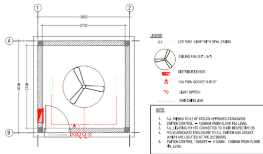
SECURE ROOM - LIGHTING & POWER LAYOUT SCALE 1:50
