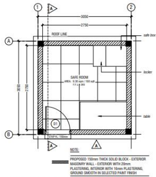
SECURE ROOM - PLAN SCALE 1:50
