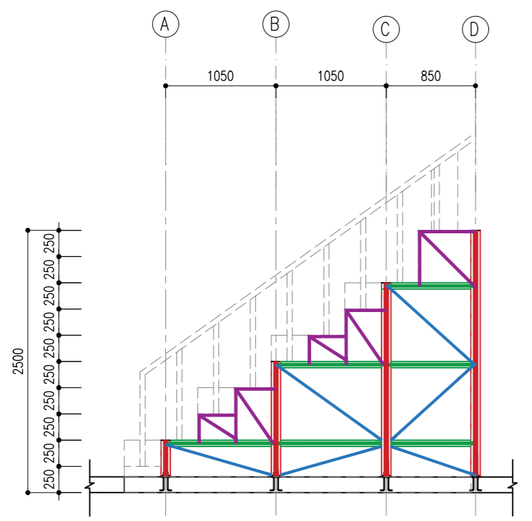
STAIR FRAME LAYOUT (SECTION A) SCALE 1: 50
