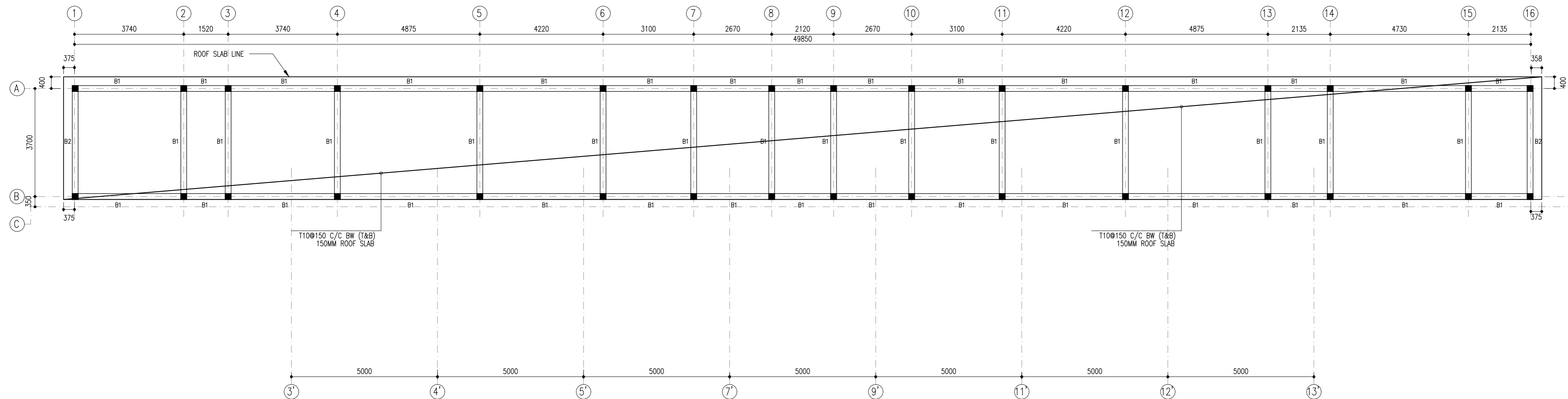
ROOF BEAM & SLAB PLAN
