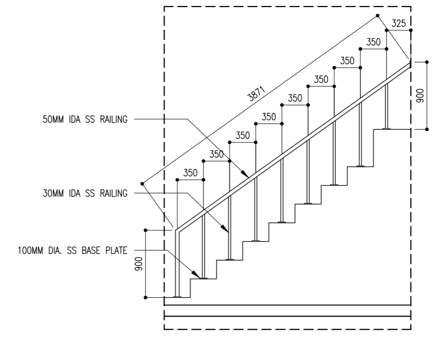
RAILING DETAILS SCALE 1: 50
