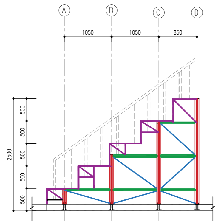
STAIR FRAME LAYOUT (SECTION B) SCALE 1: 50
