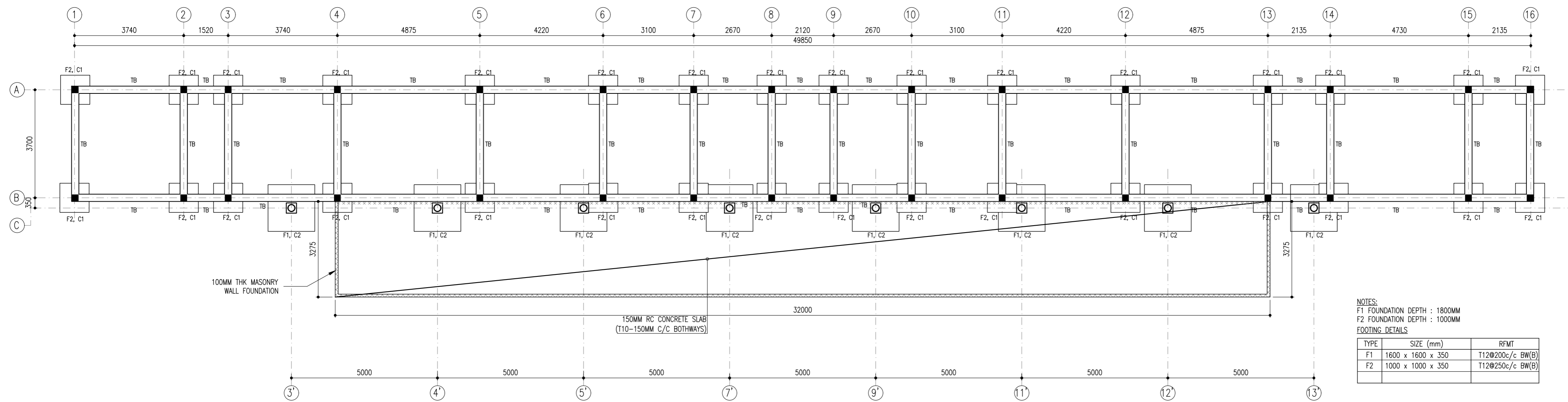
FOUNDATION & COLUMN LOCATION PLAN
