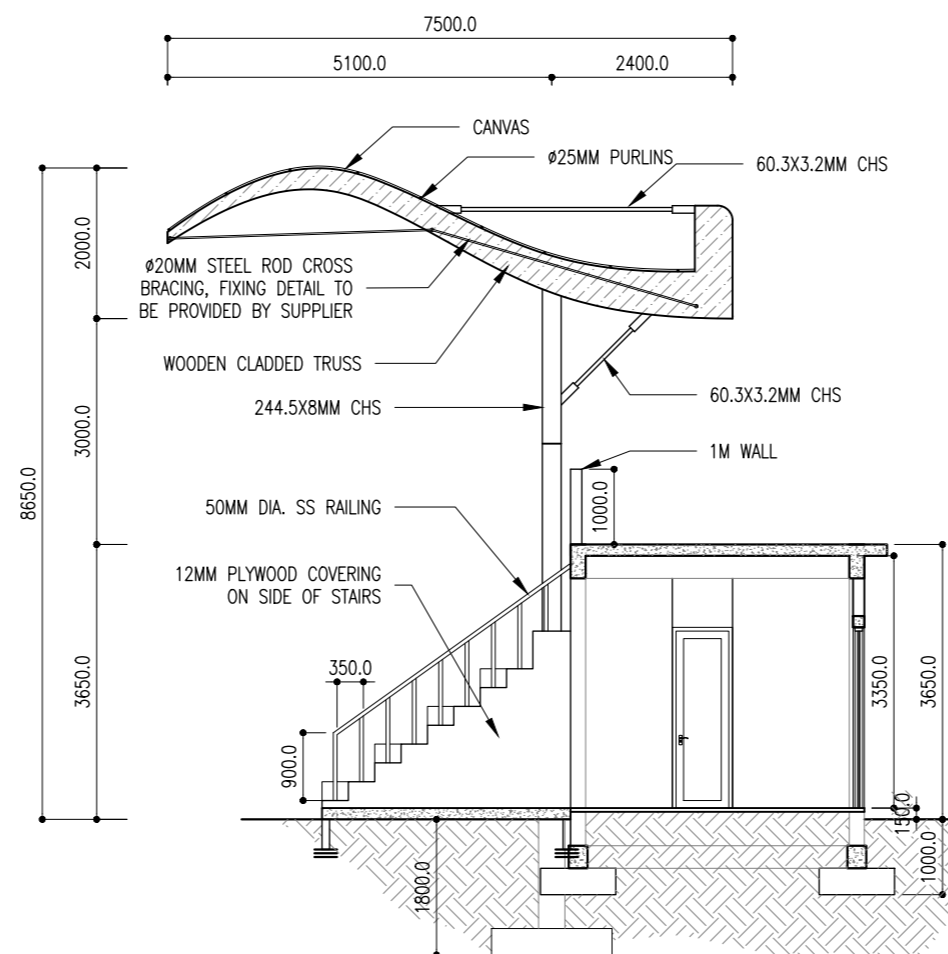
SECTION Y-Y
