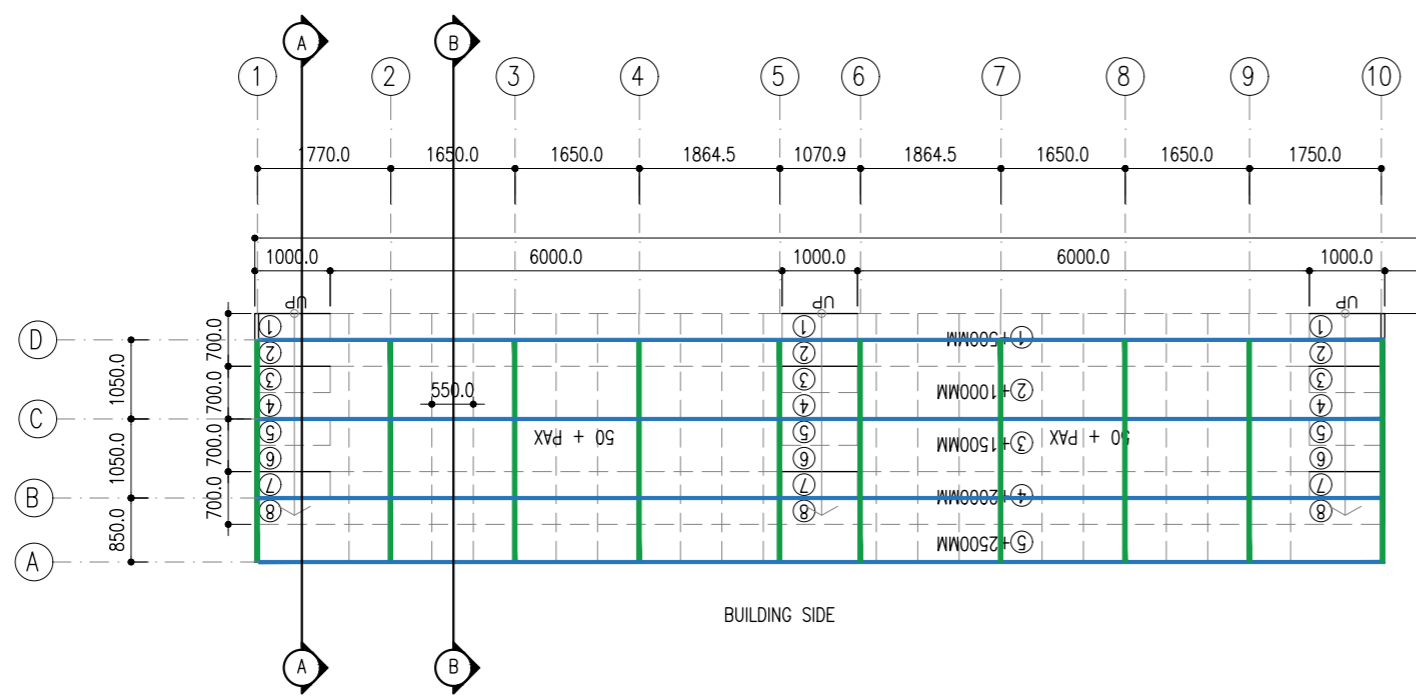
STAIR FRAME LAYOUT SCALE 1:100
