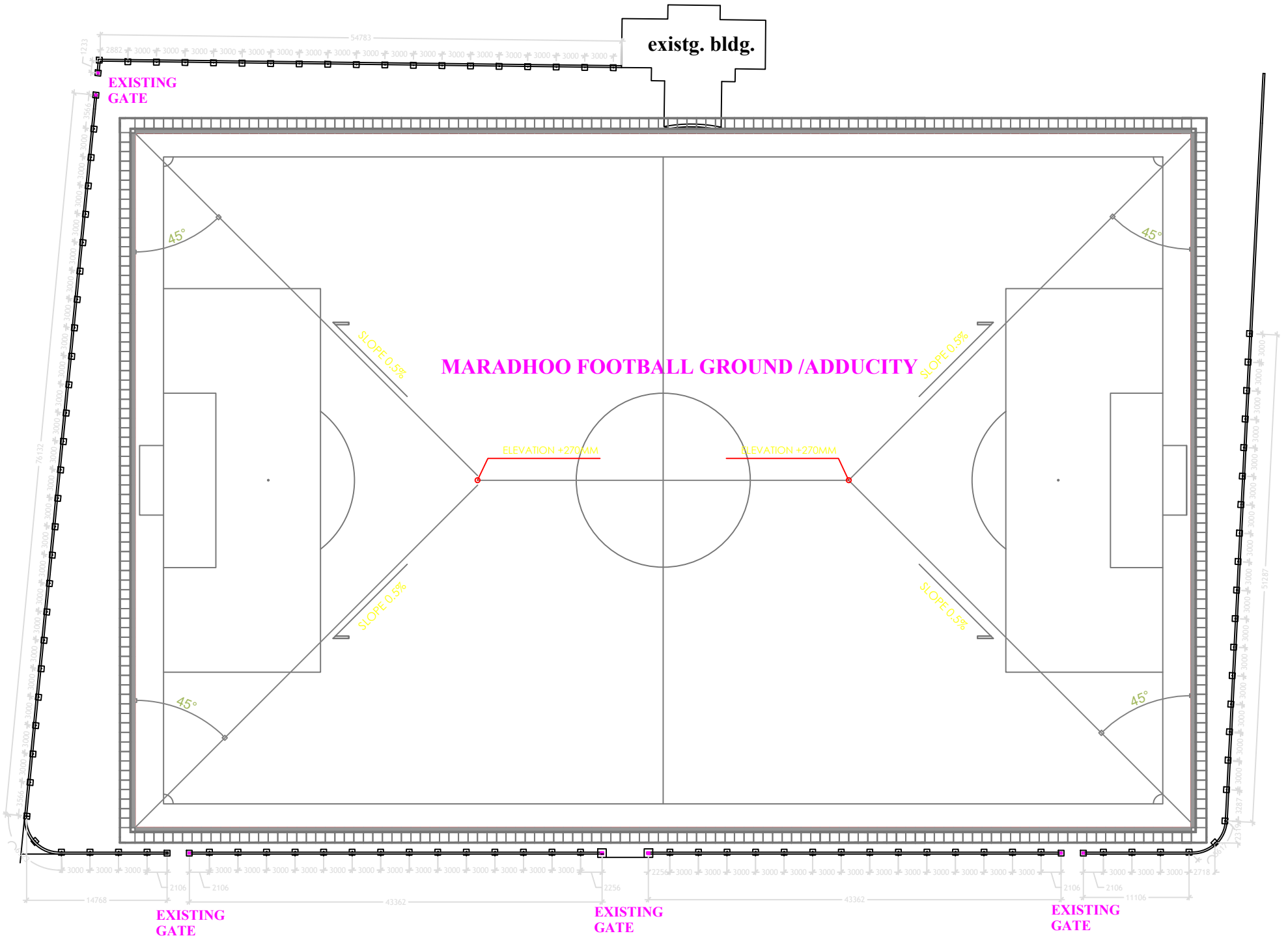
FOUNDATION /COLUMN LAYOUT PLAN
