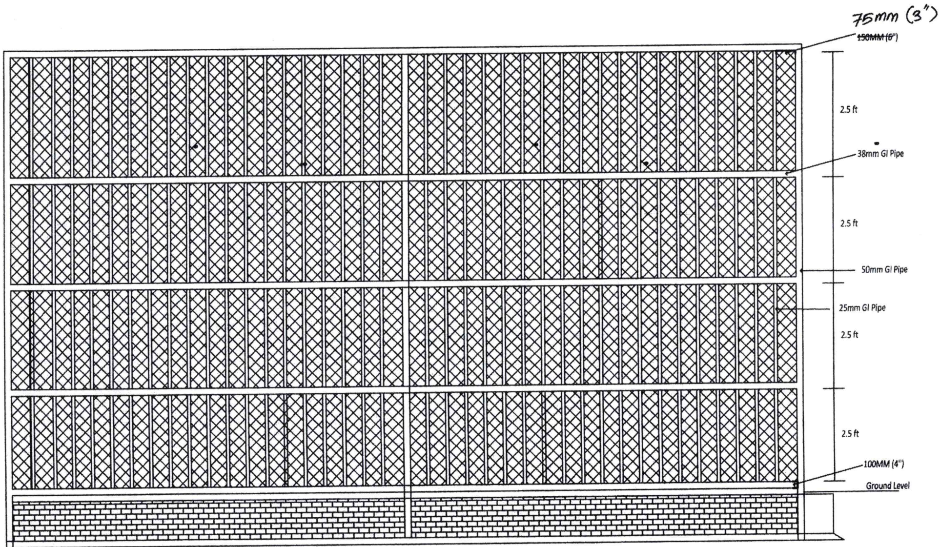
FUTSAL GROUND GOAL FENCING DETAIL SCALE 1:25
